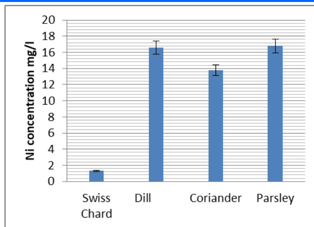
Figure (4): Comparison of nickel (Ni) concentrations in parsley, coriander, dill, and Swiss chard.
